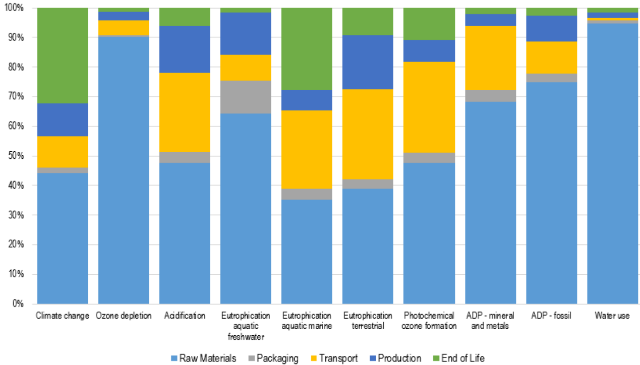
Figure 5 Graphical Impact Assessment Results for FITT NTS 3/4" Yellow
