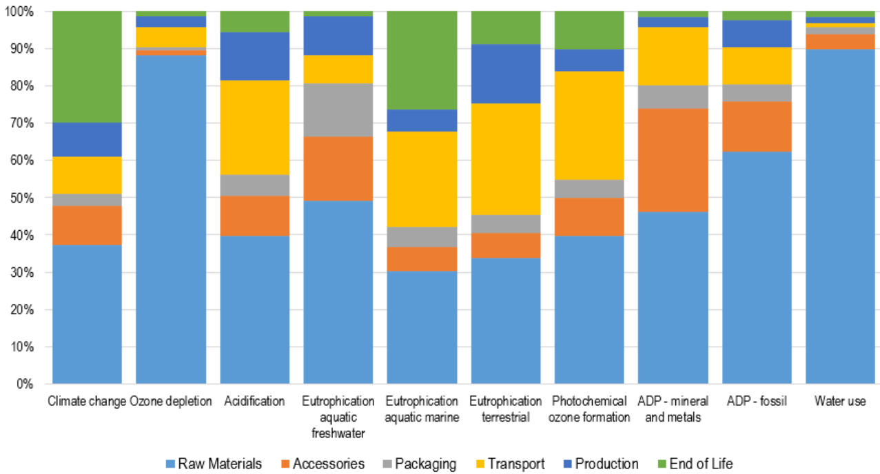
Figure 3 Graphical Impact Assessment Results for FITT NTS 5/8" KIT
