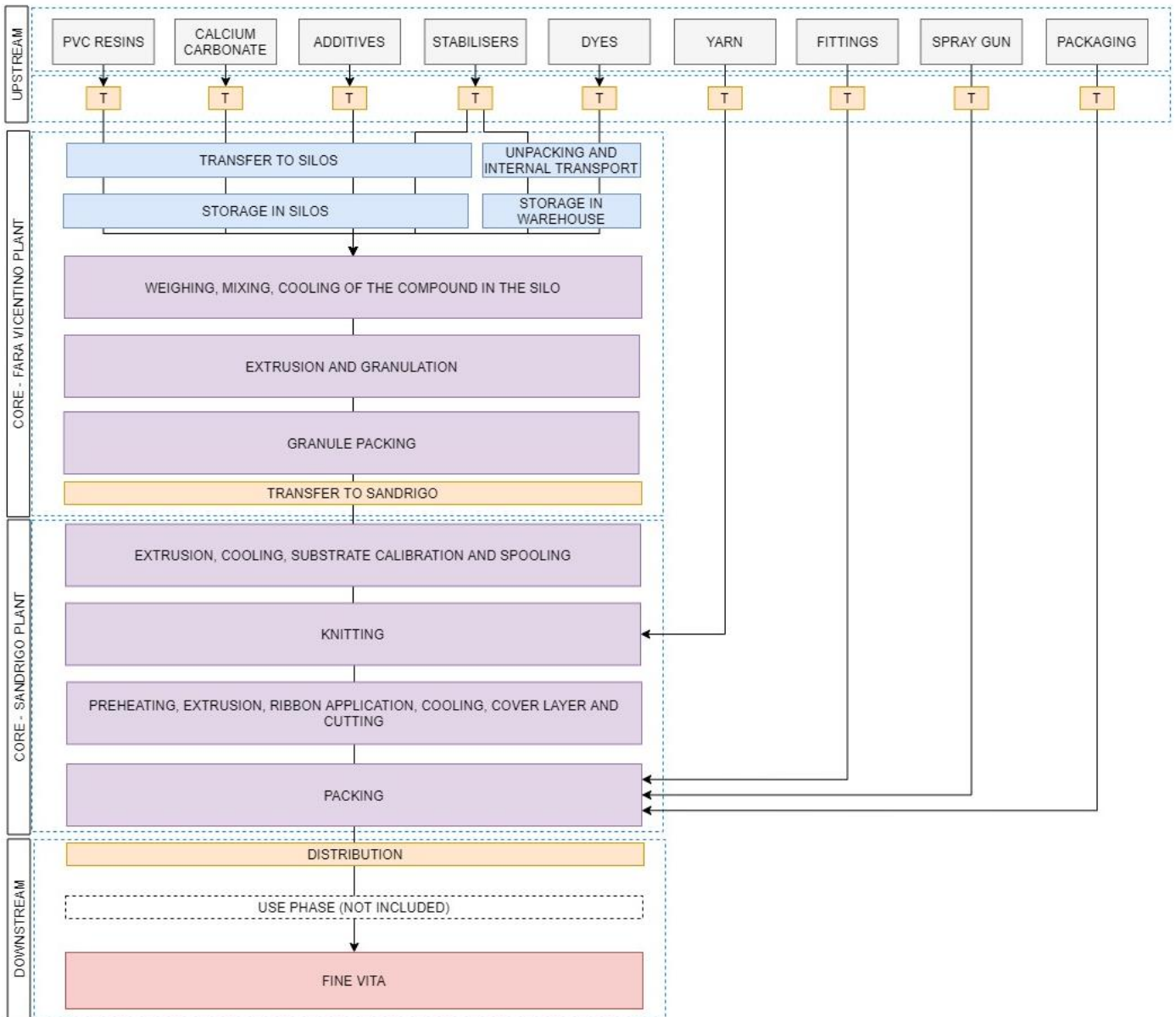
Figure 1 Diagram of the production process for FITT NTS family products
