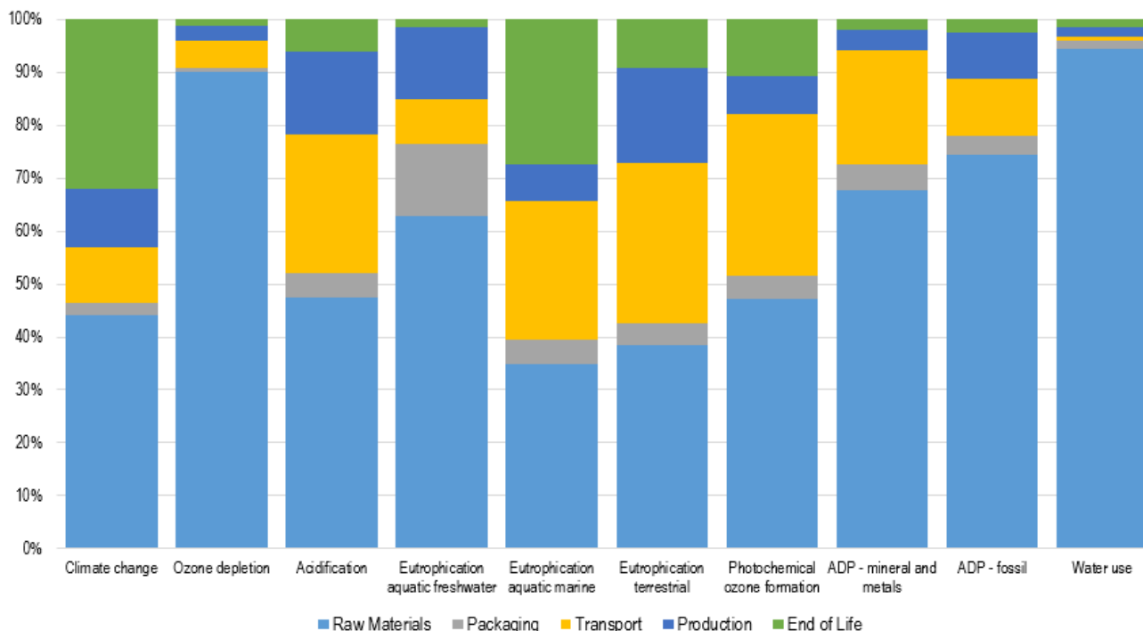
Figure 4 Graphical Impact Assessment Results for FITT NTS 5/8”
