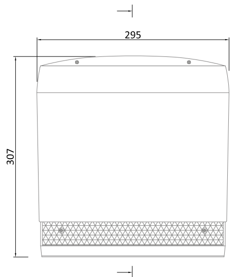
FRONT VIEW OF THE GRILLE (underside equipped with wire mesh for large insect)
