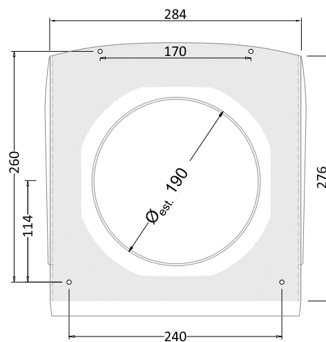
VIEW OF THE BACK OF THE GRILLE
