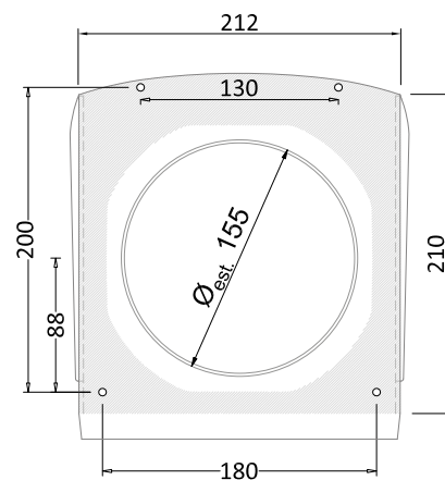
VIEW OF THE BACK OF THE GRILLE
