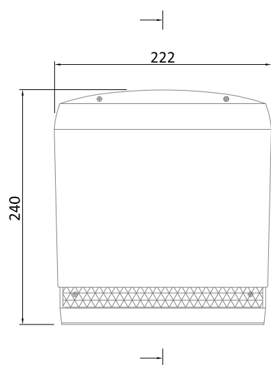
FRONT VIEW OF THE GRILLE (underside equipped with wire mesh for large insect)
