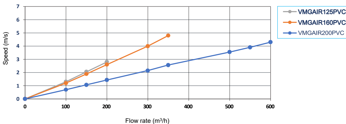
Crossing speed (m/s) for "VMGAIR-PVC" outdoor grilles at various input/output air-flow rates
