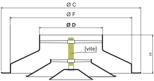
DC/08 cross-sectional view
